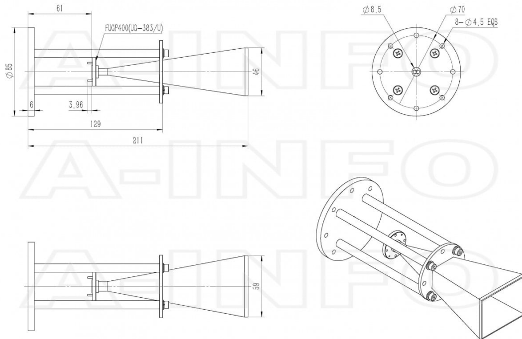
FUGP400 Output with Round Mounting Bracket (Option, P/N: LB-22-25-MB2)
