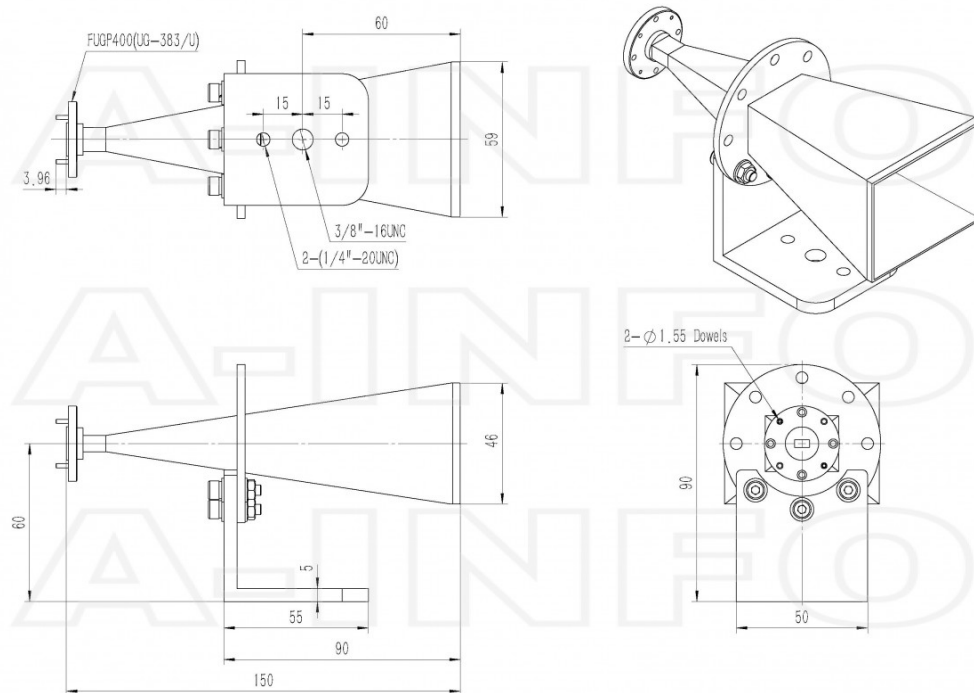
FUGP400 Output with L Type Mounting Bracket (Option, P/N: LB-22-25-L2)
